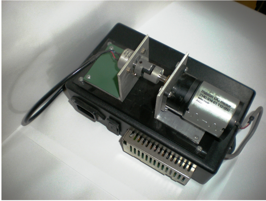
Figura 3.24: Motor CC Maxon F2140.
